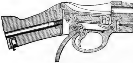
MARTINI-HENRY RIFLE.
